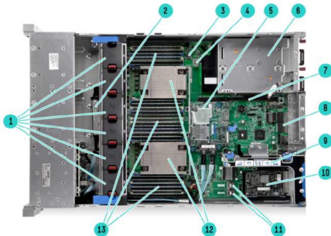
Internal View
