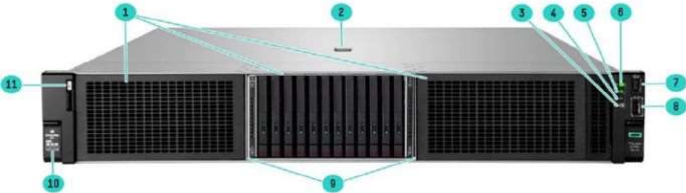
Front View -12EDSFF chassis shown
