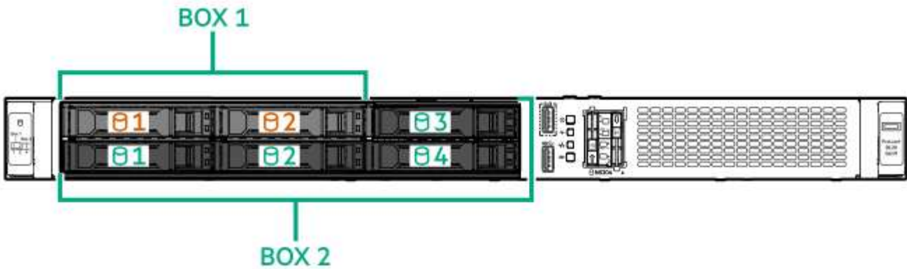
4 SFF + 2SFF device bay numbering
