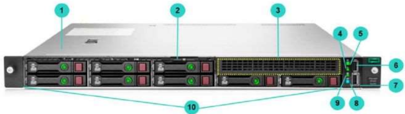
8 SFF chassis - Front View
