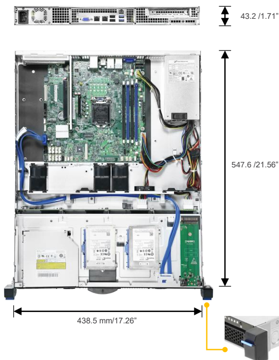
Rack Handle(Optional)
