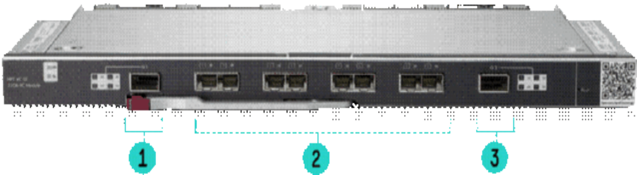
HPE Synergy VC SE 32Gb FC Module Front View
