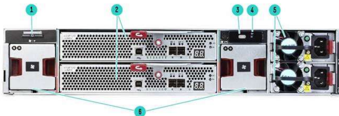
HPE D3000 Enclosure (Large and Small Form factor Features) Rear Panel components
